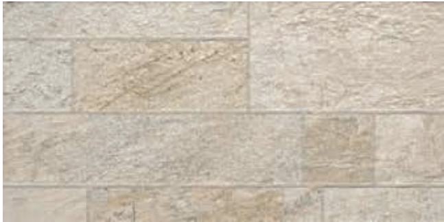
30x60 cm 11 7/8 "x23 5/8 " SDL560 SPESSORE 10 MM R12 / A+B+C ASTM C1028 > 0,70 DRY ≥ 0,60 WET
